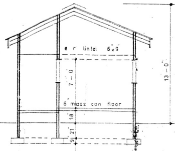
CROSS SECTION
